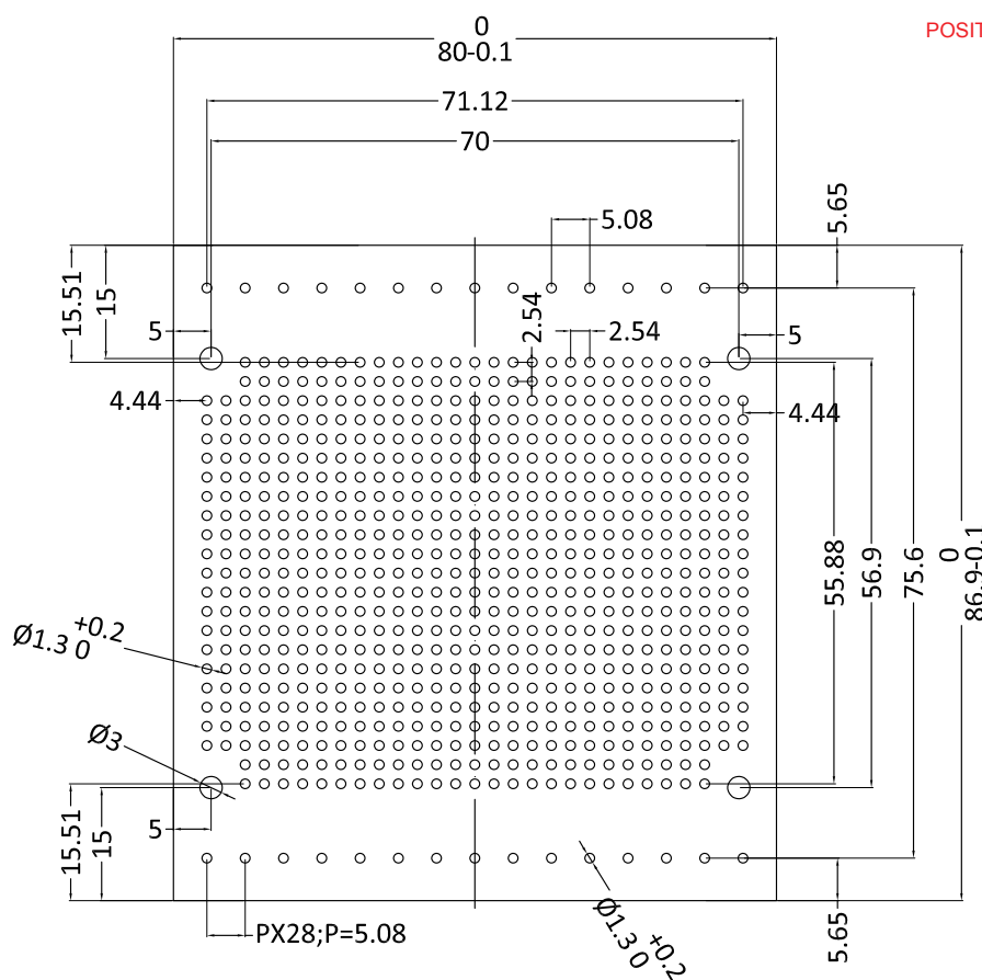
PCB of position "A" for RND 455-00560
