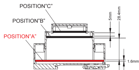
PCB of position "A" for RND 455-00560
